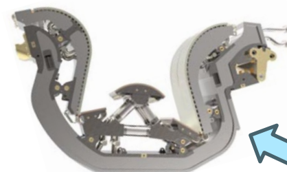
Divertor Cassette
